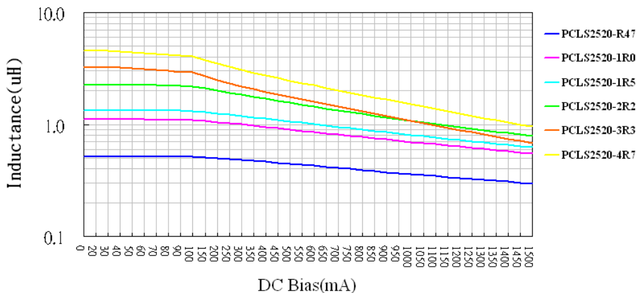
Inductance VS DC bias current
