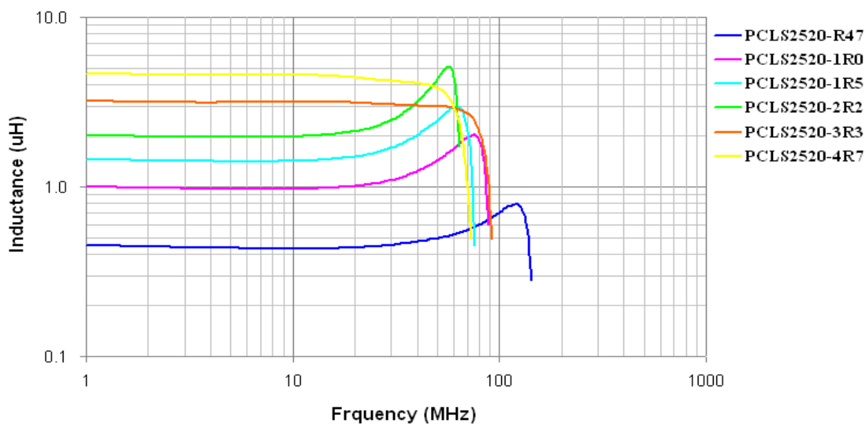
Inductance vs Frequency
